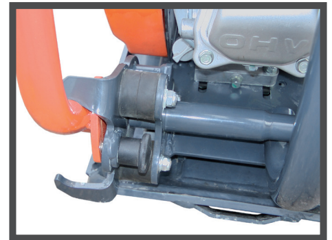
HANDLE LATCH FOR INCREASED STABILITY WHILST OPERATING THE WHEEL KIT
